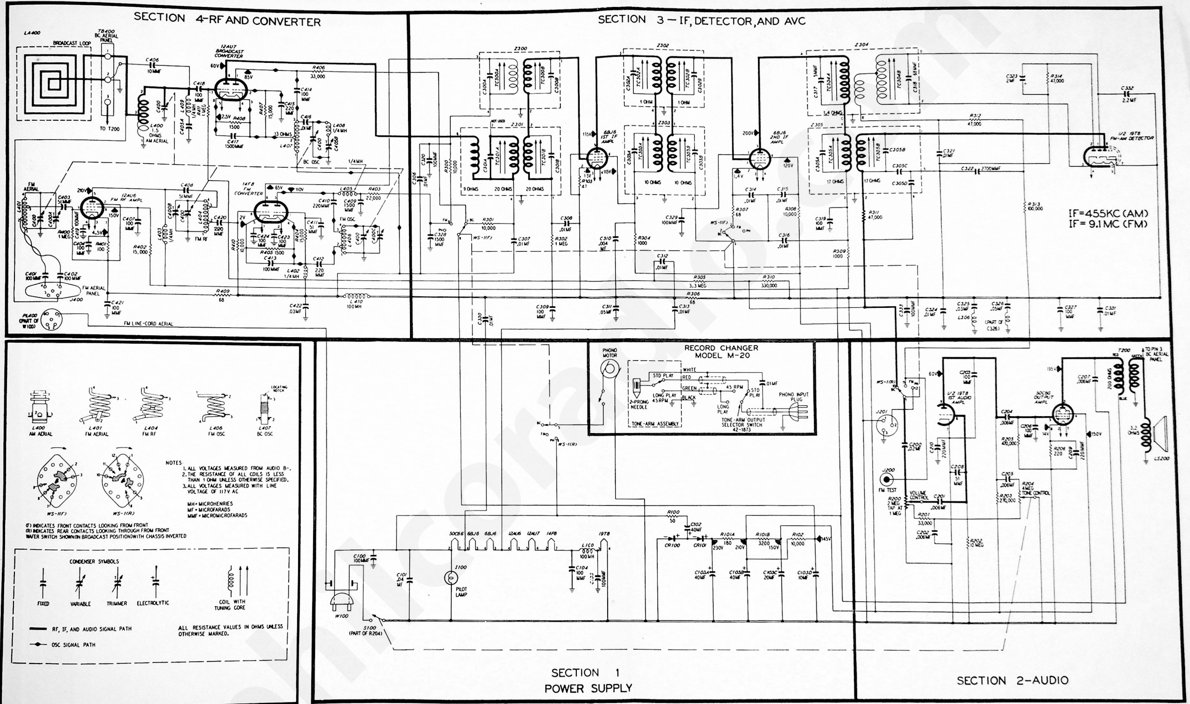
Figure 1. Philco Radio-Phonograph Model 50-1720, Schematic Diagram
